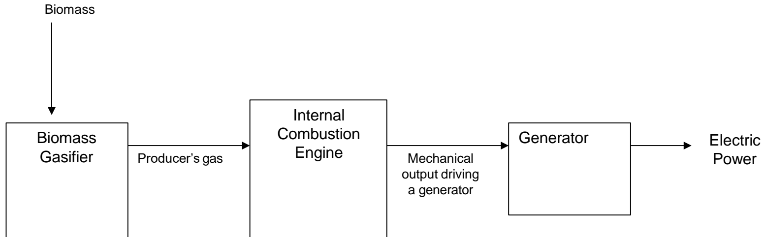
Figure 6: Block diagram of a producer's gas electricity system
