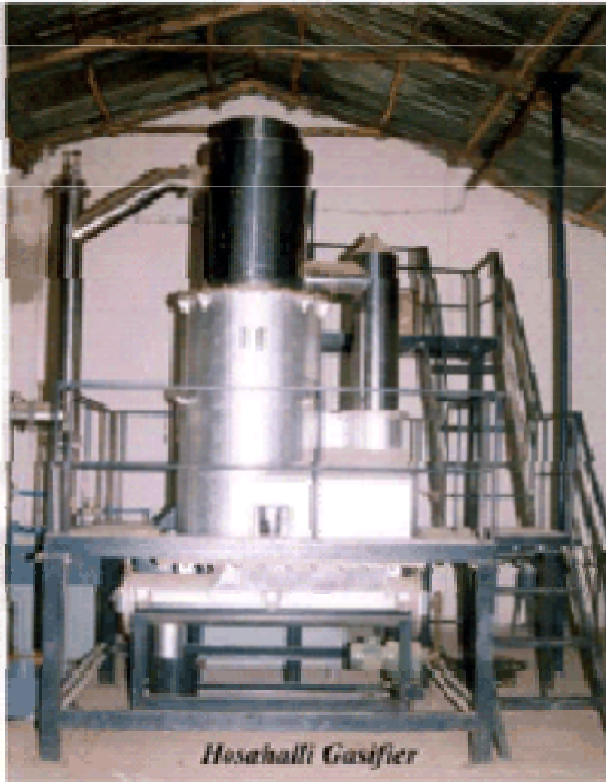
Fig 8: Biomass Gasifier Installed in Hosahalli, Karnataka.
